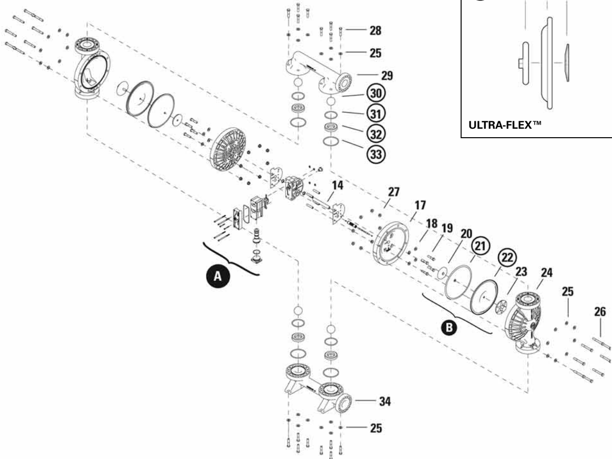
CENTER-PORTED
