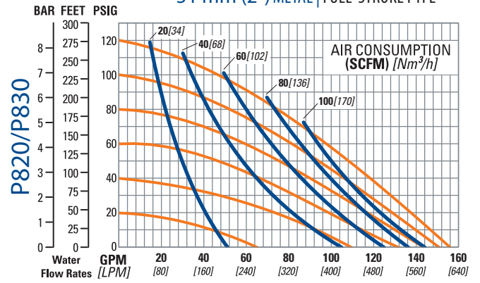
51 mm (2") METAL | FULL-STROKE PTFE
